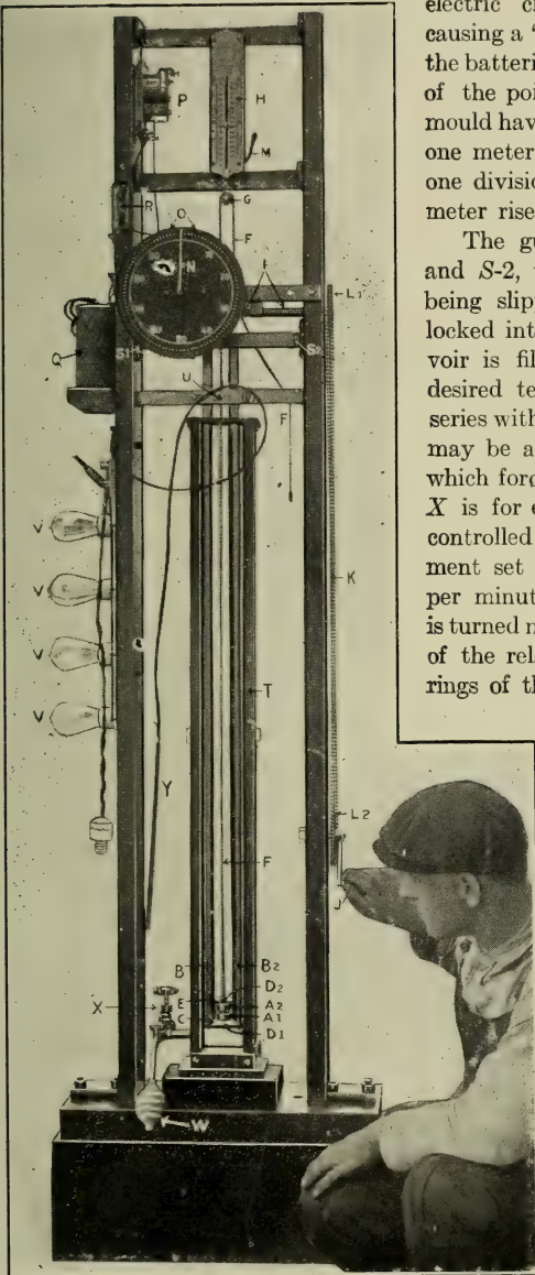
FIG. 170.—Tensometer.
